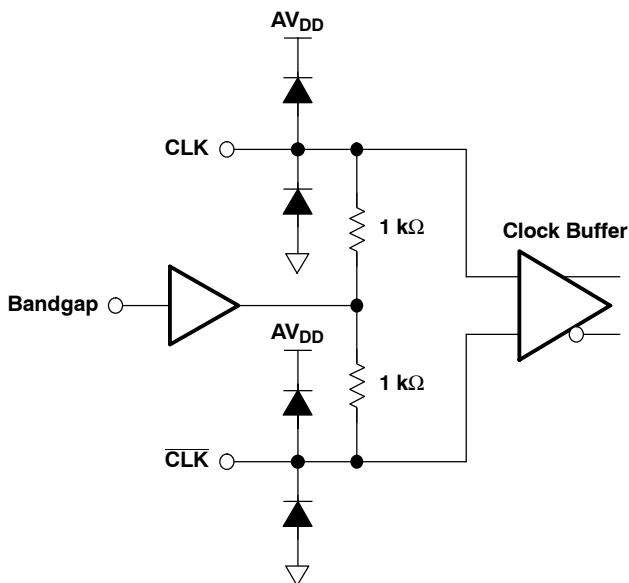
Figure 34. Clock Input
